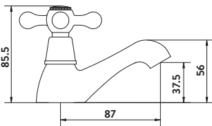
Basin Taps
