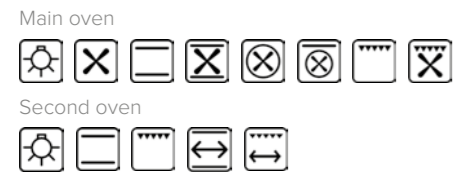
RV1002 100cm twin cavity range cooker, electric ovens, gas hobs
